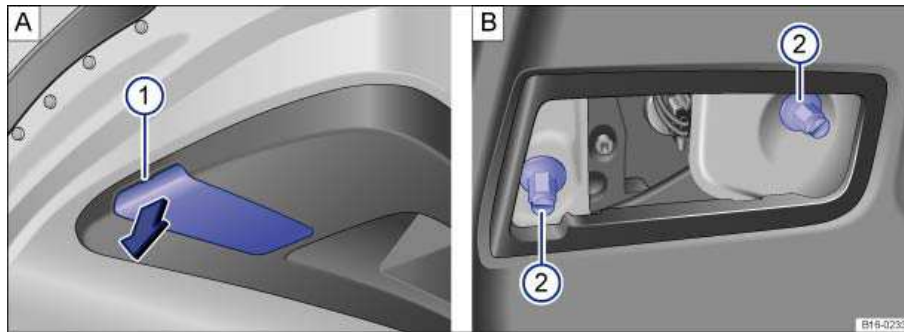
Fig. 182 In the luggage compartment lid: A: removing the cover on the LED taillight, B: Removing the LED taillight.
