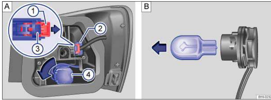
Fig. 187 LED taillight: A: removing the bulb holder, B: removing the bulb.
