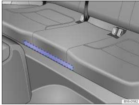
Fig. 127 Air ventilation for the high-voltage battery under the rear seat bench.
