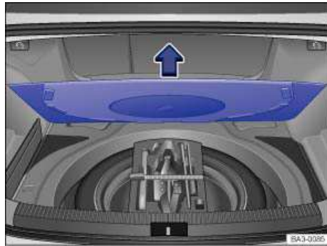
Fig. 162 In the luggage compartment under the floor panel: Compact spare wheel and vehicle tool kit.
