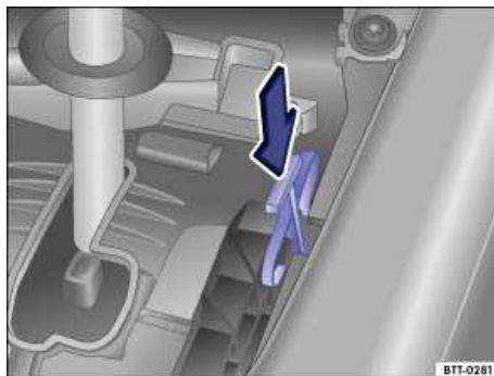
Fig. 161 Releasing the selector lever lock.
