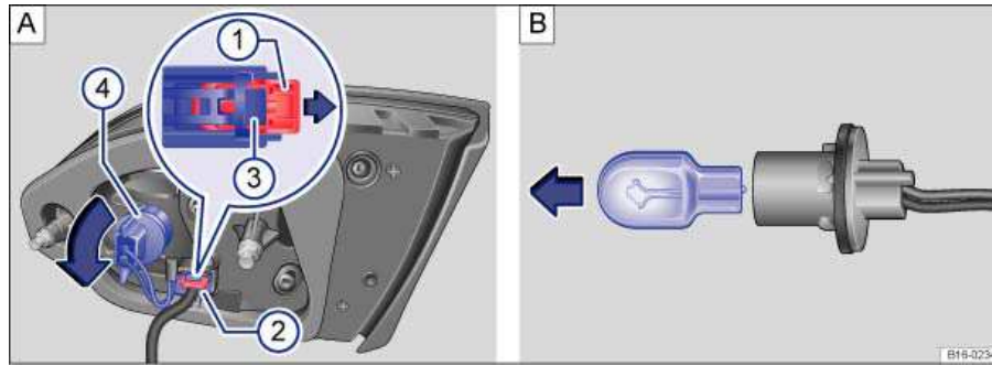
Fig. 183 LED taillight: A: Removing the bulb holder, B: Removing the bulb.
