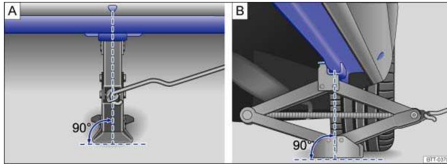
Fig. 170 Jack in position at the left rear lift point.
