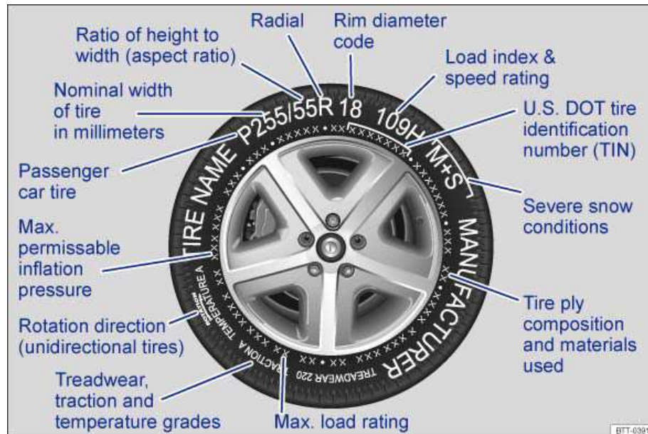
Fig. 95 International tire labeling.
