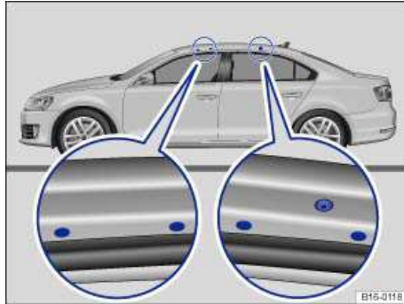
Fig. 89 Attachment points for the base carrier and roof rack.
