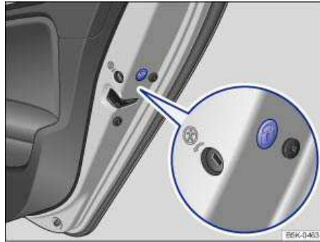
Fig. 154 On the front side of the right rear door: Emergency lock, covered by a rubber seal.
