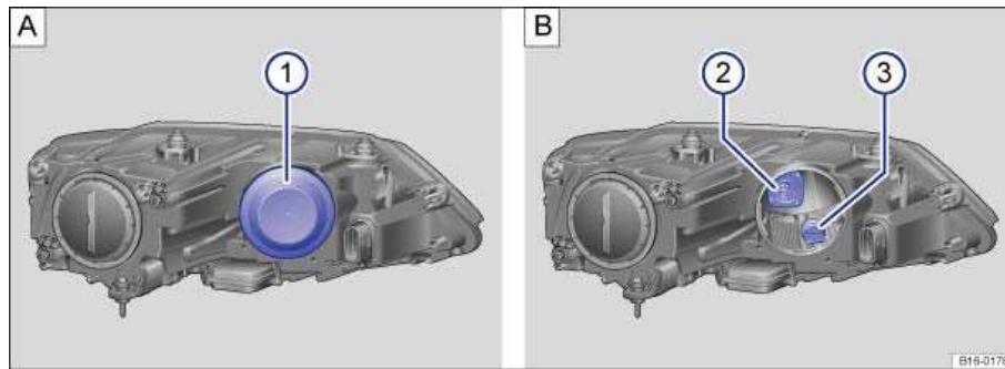
Fig. 177 In the engine compartment: Cover 1 on the left headlight for the cornering light bulb holder 2 and the turn signal bulb holder 3.
