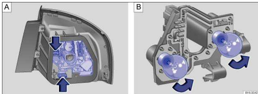
Fig. 185 Taillights: A: Removing the bulb holder. B: Removing the taillight bulbs.
