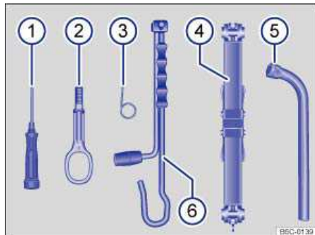
Fig. 163 Contents of the vehicle tool kit.
