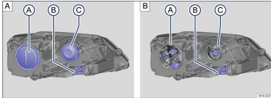
Fig. 176 In the engine compartment: Covers in the left headlight assembly. A Low beam headlight, daytime low beam headlight or daytime running light, side marker light; B Turn signal indicator; C High beam, parking light, daytime running light.
