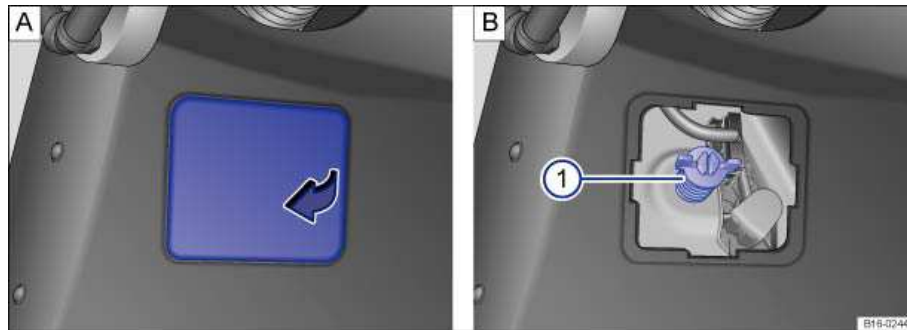
Fig. 186 In the side of luggage compartment: A: Open cover of the rear side panel. B: Removing the LED taillight assembly.
