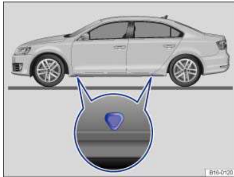
Fig. 169 Lift points for the jack.
