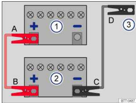
Fig. 189 Diagram for attaching the jumper cables: Dead battery 1 and booster battery 2.
