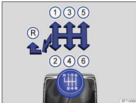
Fig. 126 Gearshift pattern of a 6-speed manual transmission.
