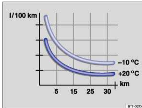
Fig. 135 Fuel consumption in l/100 km at 2 different outside air temperatures.
