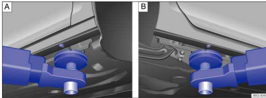
Fig. 162 A: Lifting point at the front. B: Lifting point at rear for lifting the vehicle using a workshop hoist or floor jack.
