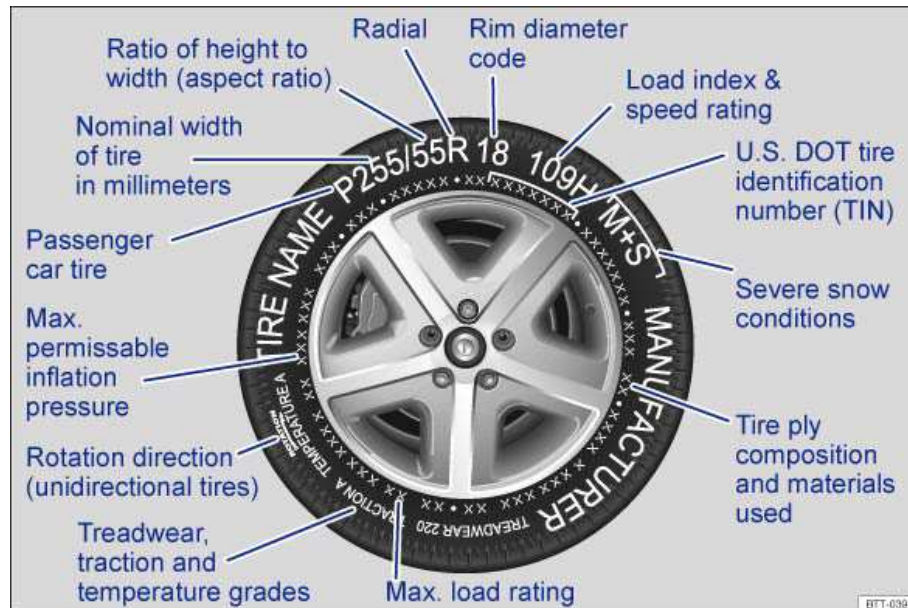
Fig. 105 International tire labeling.
