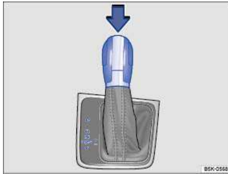
Fig. 127 Automatic transmission selector lever with shift lever release button (arrow).
