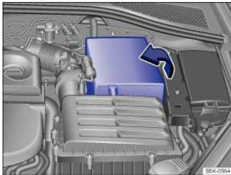
Fig. 159 In the engine compartment: Open the sleeve covering of the vehicle battery.
