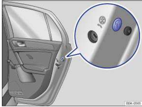
Fig. 165 On the front side of the right rear door: Manual lock, covered by a rubber seal.
