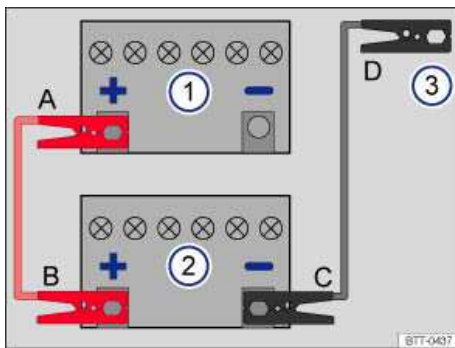
Fig. 187 Diagram for attaching the jumper cables: Dead battery 1 and booster battery 2.
