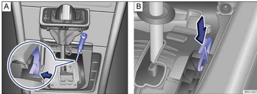
Fig. 170 Releasing the selector lever lock (versions A and B).
