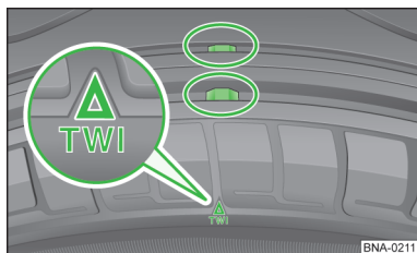
Fig. 65 Tread: wear indicator
