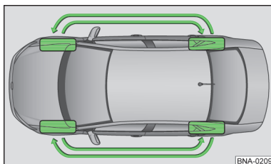
Fig. 63 Pattern for the exchange of the wheels
