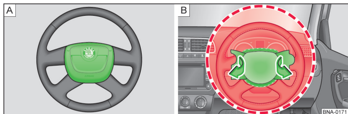
Fig. 26 Installation position and deployment area of the driver's front airbag
