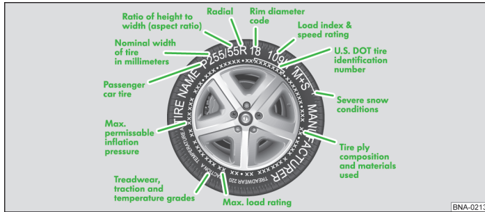
Fig. 67 International tyre inscription
