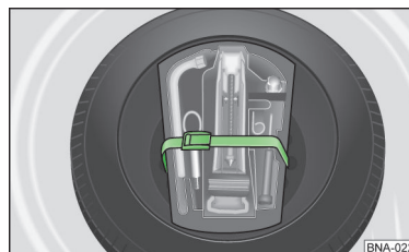
Fig. 74 In the luggage compartment below the floor covering: spare wheel and tool kit in the foam part
