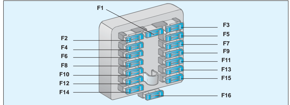
16 fuse box
