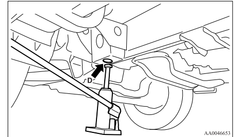
D- Front jacking point (2WD vehicles 16 inch wheels and 4WD vehicles)
