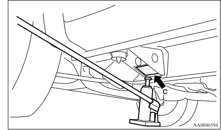
C- Front jacking point (2WD vehicles with 15 inch wheels)
